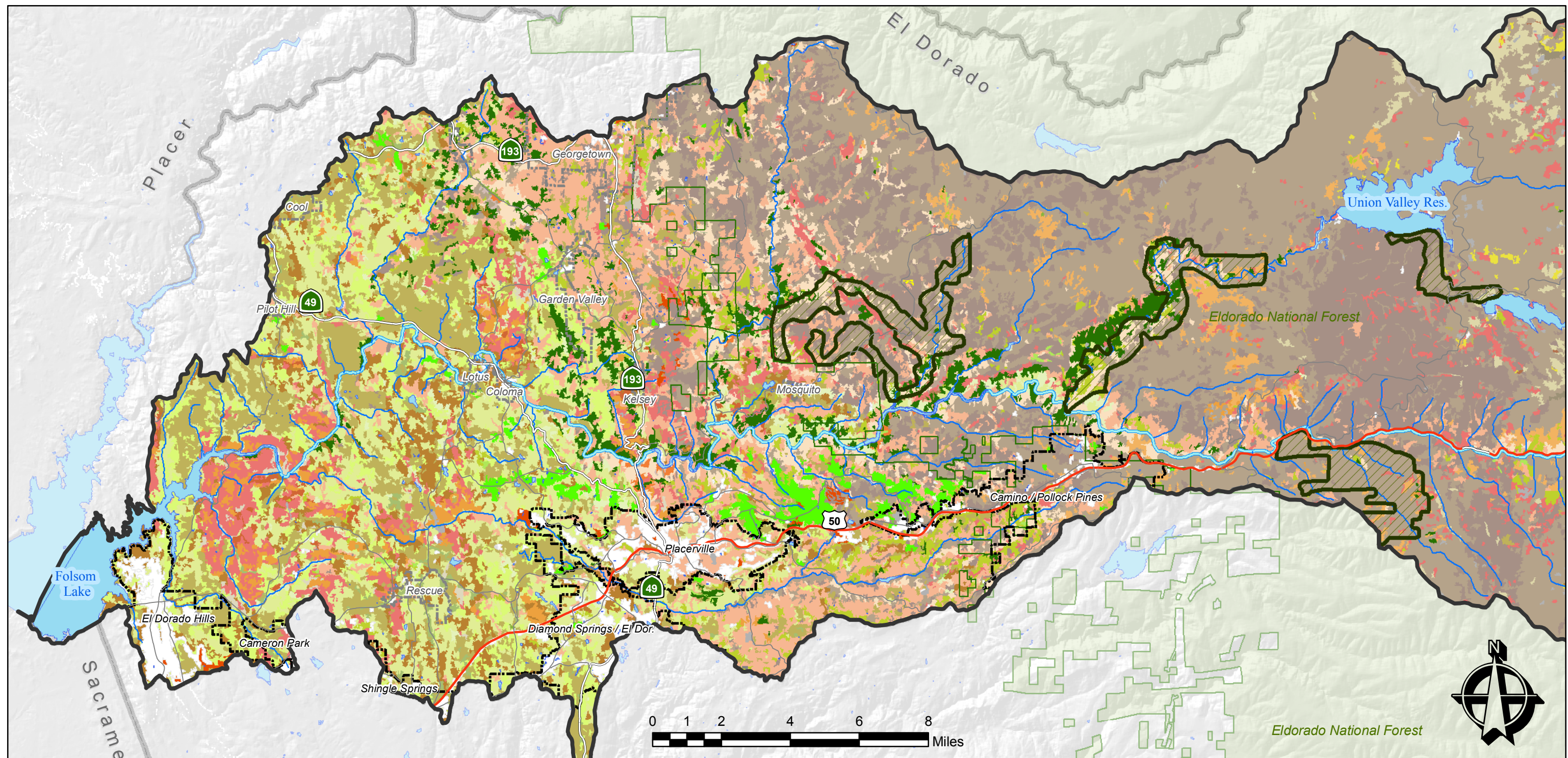
Figure 2-5. Vegetation Types - West South Fork American River Watershed Plan
